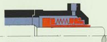
single mechanical seal garniture mécanique simple
