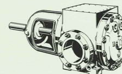
fig. 9 pump with integral heating jacket
